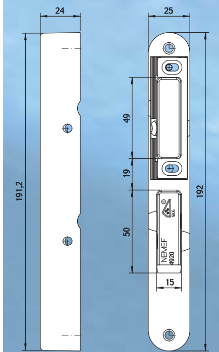
VS 4920 (Excellence line)
