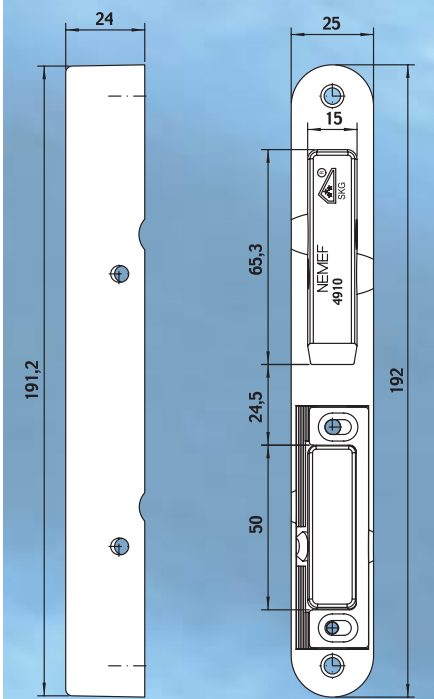
VS 4910 (Comfort line)
