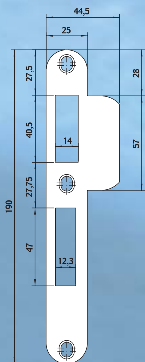
PM 4920 (Excellence line)
