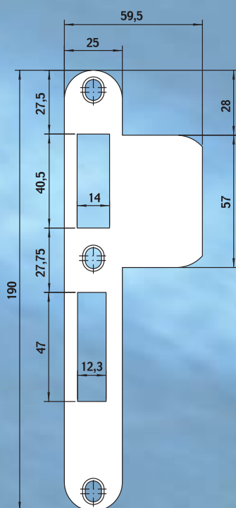
VPM 4920 (Excellence line)
